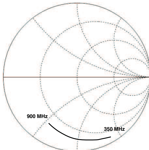
Figure 35. UHF RFIN
