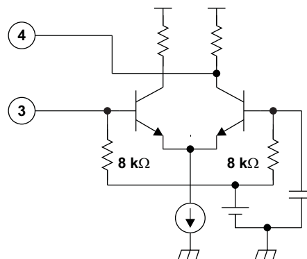
Figure 18. VHI OSC B and VHI OSC C
