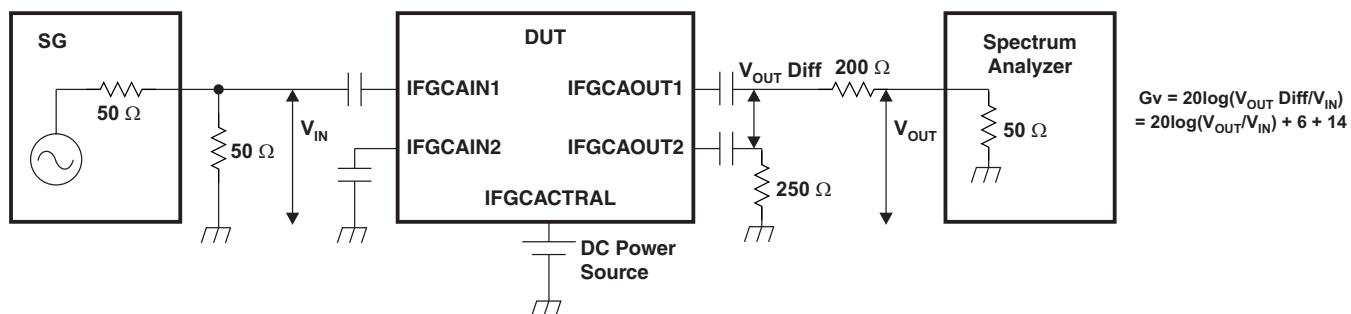
Figure 30. IF GCA Gain Measurement Circuit
