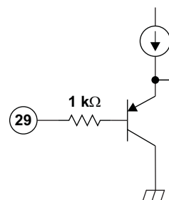
Figure 14. SCL
