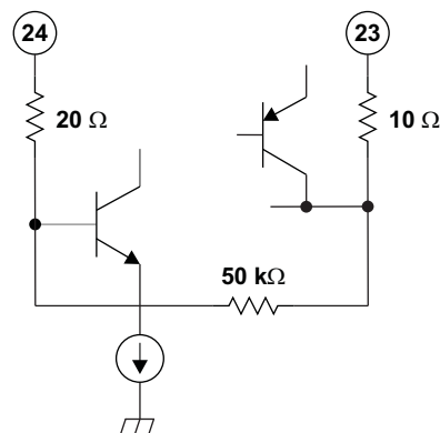
Figure 22. XTAL1 and XTAL2
