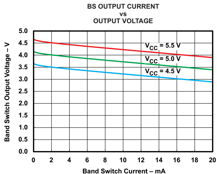
Figure 33. Band Switch Driver Output Voltage
