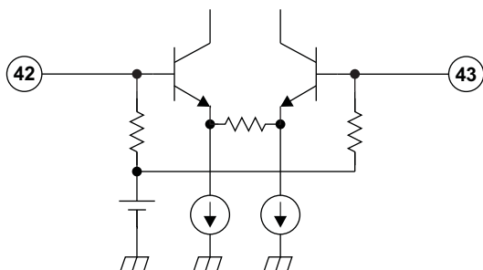
Figure 17. UHF RF IN1 and UHF RF IN2
